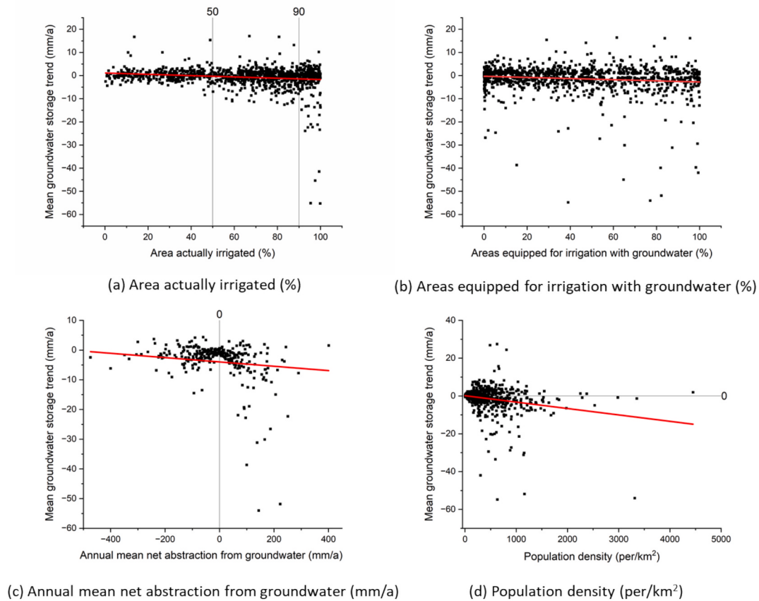
Fig. 8. Mean GWS plotted against four possible factors of human impact, (a) area actually irrigated (%), (b) areas equipped for irrigation with groundwater (%), (c) annual mean net abstraction from groundwater (mm/a), and (d) population density (per/km 2 ).
